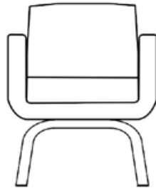
W 670mm D 600mm H 765mm SH 465mm MYNI CHAIR Curved mild steel leg powdercoated
